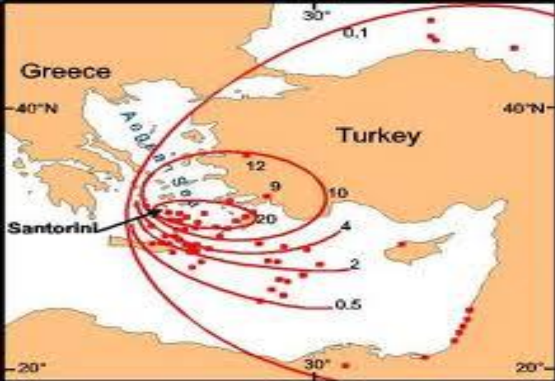
Ash from the Minoan eruption (in cm)
